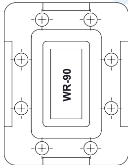
WR-90 WAVEGUIDE CPR-90G GROOVED FLANGE
