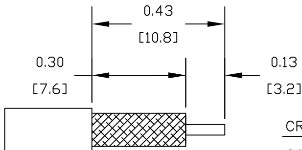
STRIPPING DIMENSIONS
