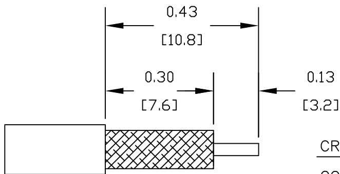
STRIPPING DIMENSIONS
