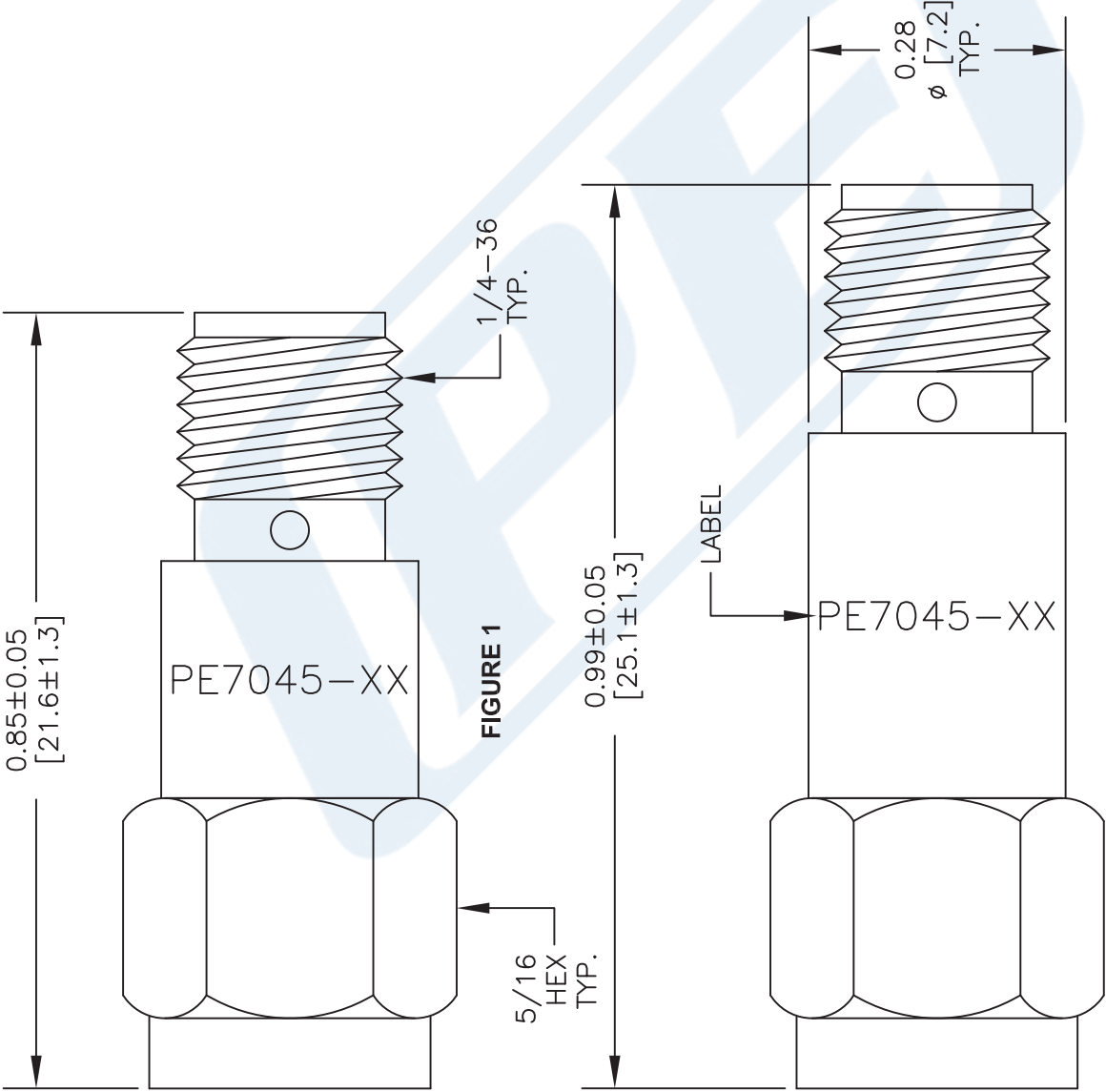
SMA FEMALE
