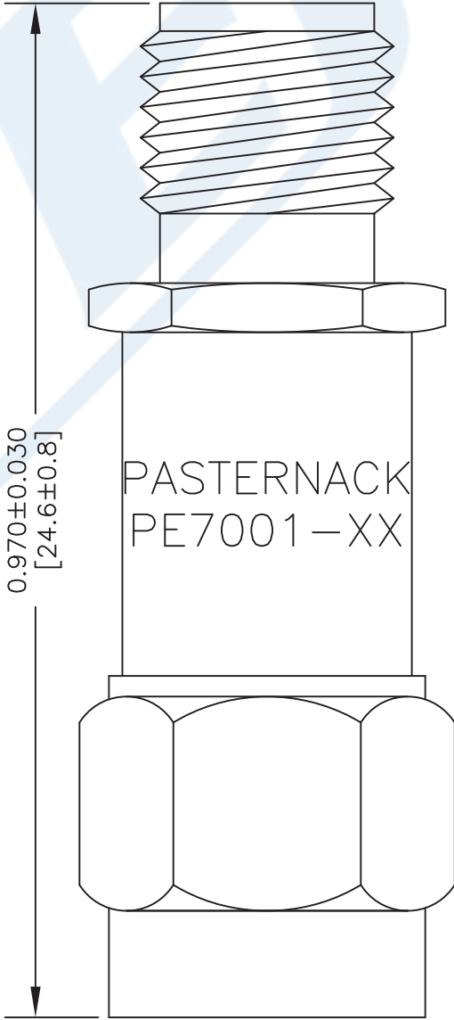
SMA FEMALE
