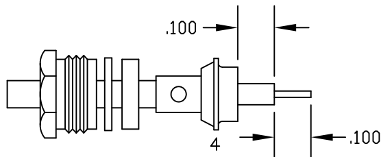
ASSEMBLY (B)
