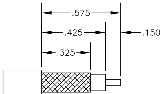
STRIPPING DIMENSIONS
