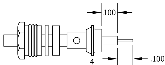
ASSEMBLY (B)
