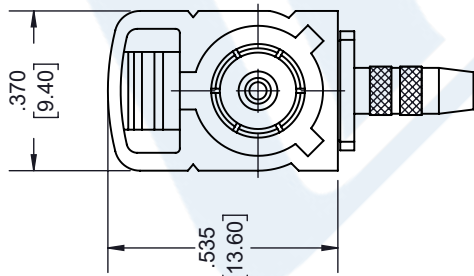
FAKRA JACK RA K CODING CURRY
