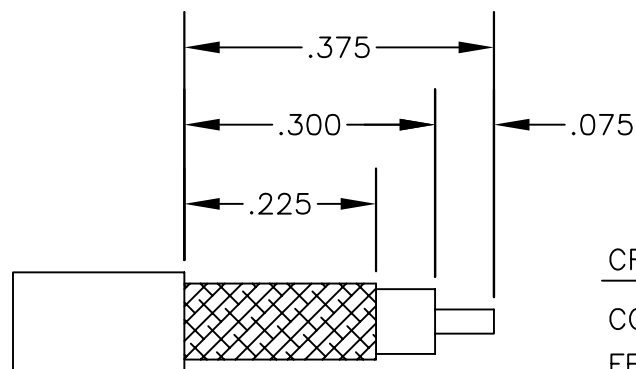
STRIPPING DIMENSIONS
