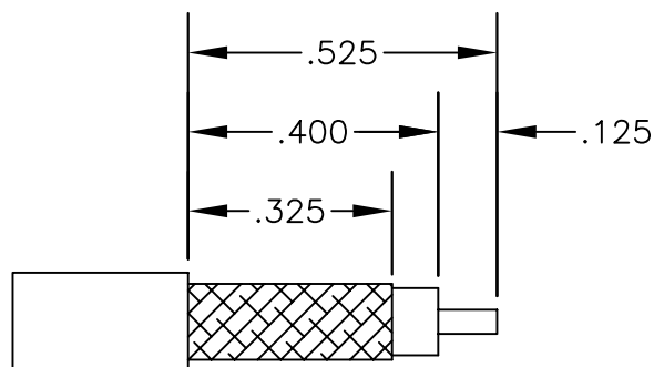
STRIPPING DIMENSIONS
