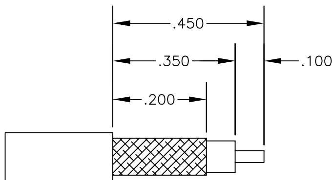
STRIPPING DIMENSIONS
