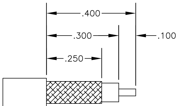
STRIPPING DIMENSIONS
