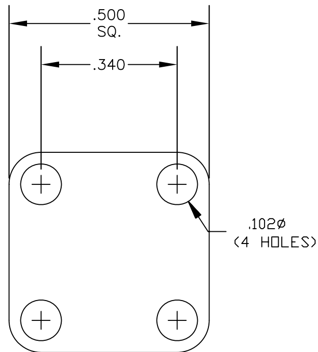
MOUNTING HOLES
