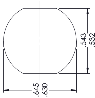
MOUNTING HOLE
