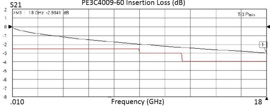
PE3C4009-60 Insertion Loss (dB)
