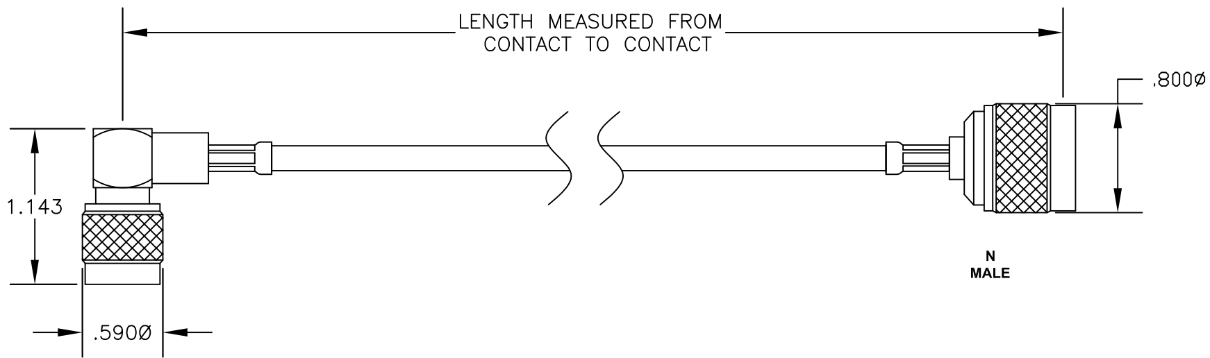
REVERSE POLARITY TNC MALE RIGHT ANGLE
