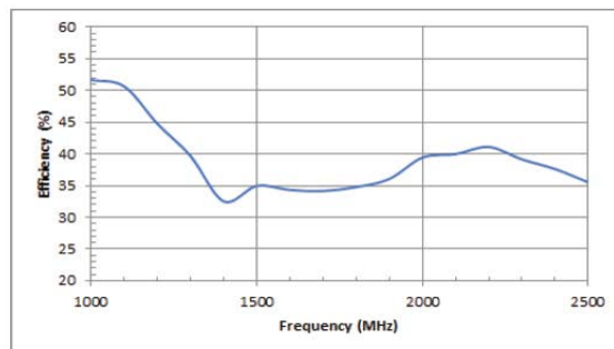
Efficiency
