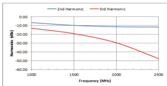
Harmonics (@ Psat)
