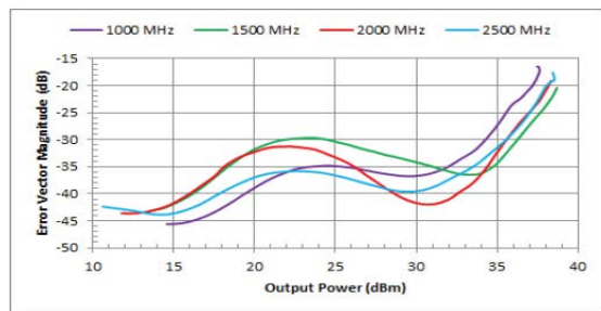
Error Vector Magnitude (dB) [w/ 16QAM Waveform]
