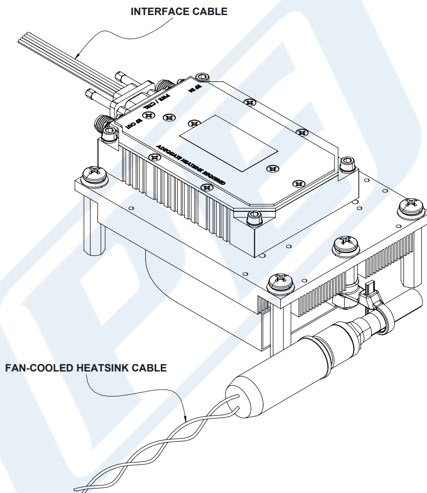
illustration of Amplifier & Heatsink.
