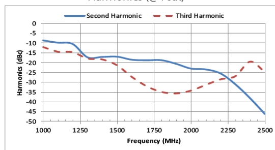
Harmonics (@ Psat)
