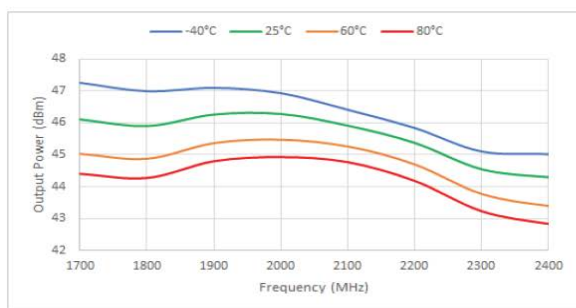
Output Power vs. Temperature [Baseplate]
