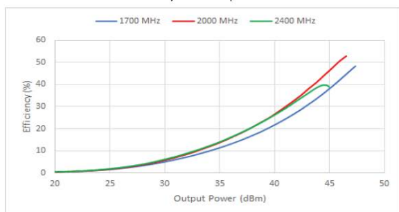
Efficiency vs. Output Power
